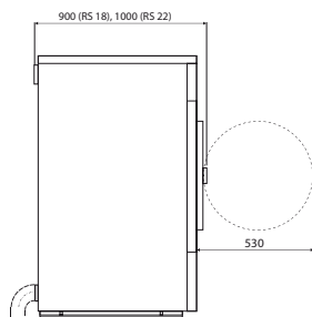
SIDE RS 18 22
