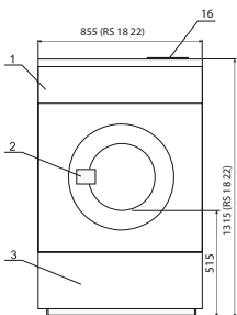
FRONT RS 18 22
