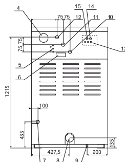
BACK RS 18 22
